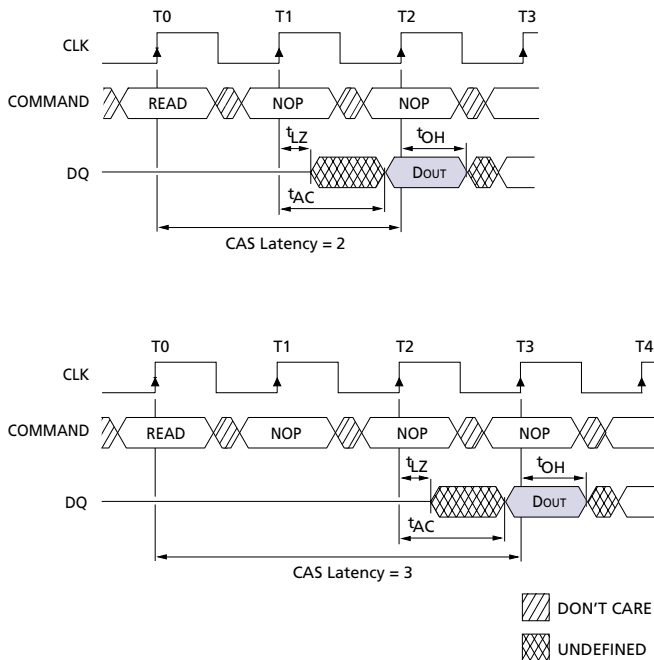
Figure 1 CAS Latency
