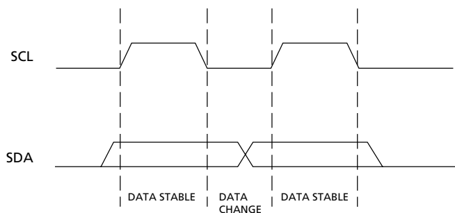
Figure 3 Data Validity
