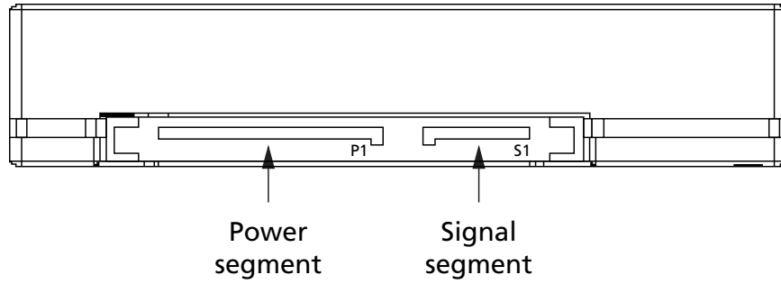
Figure 3: SSD Interface Connections
