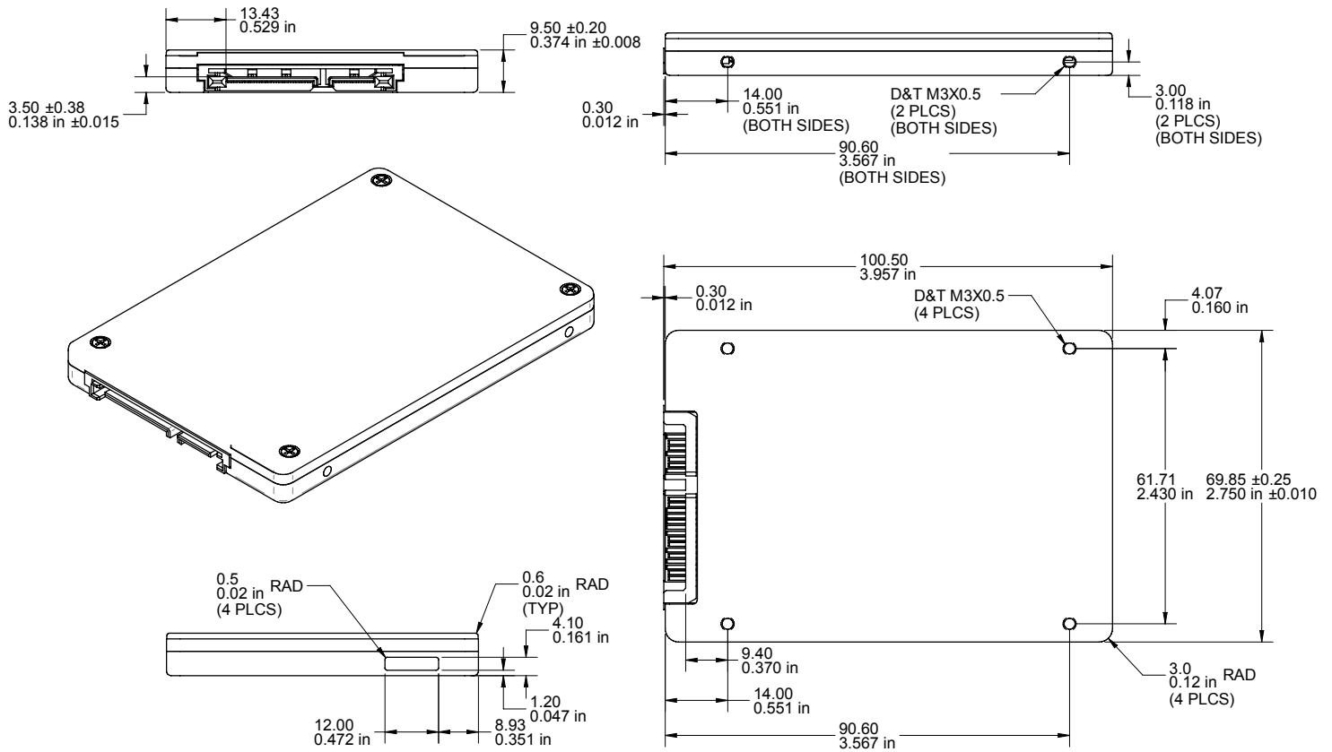
Figure 4: 2.5-Inch Package (Preliminary)
