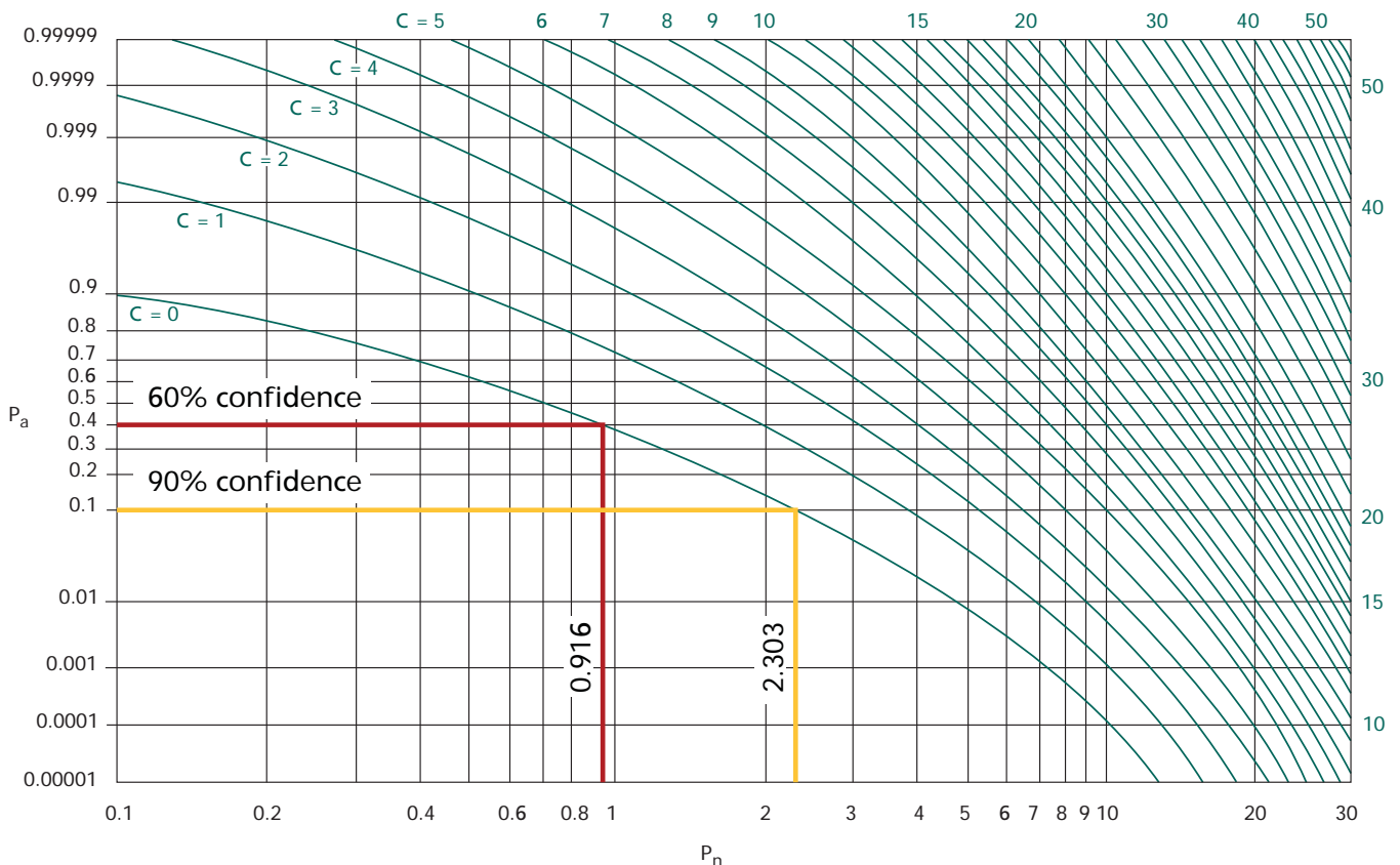
Figure 2: Poisson Curves
