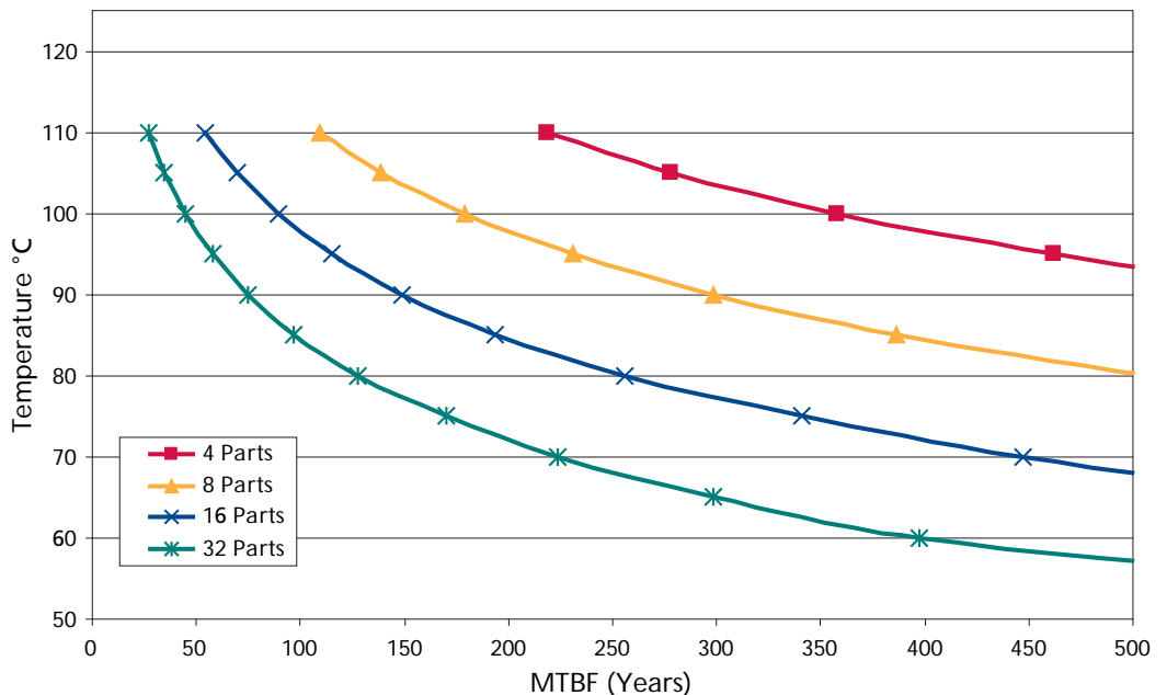
Figure 3: Example of Memory System Mean Time Between Failure for Micron Multiple 256Mb SDRAM Components
