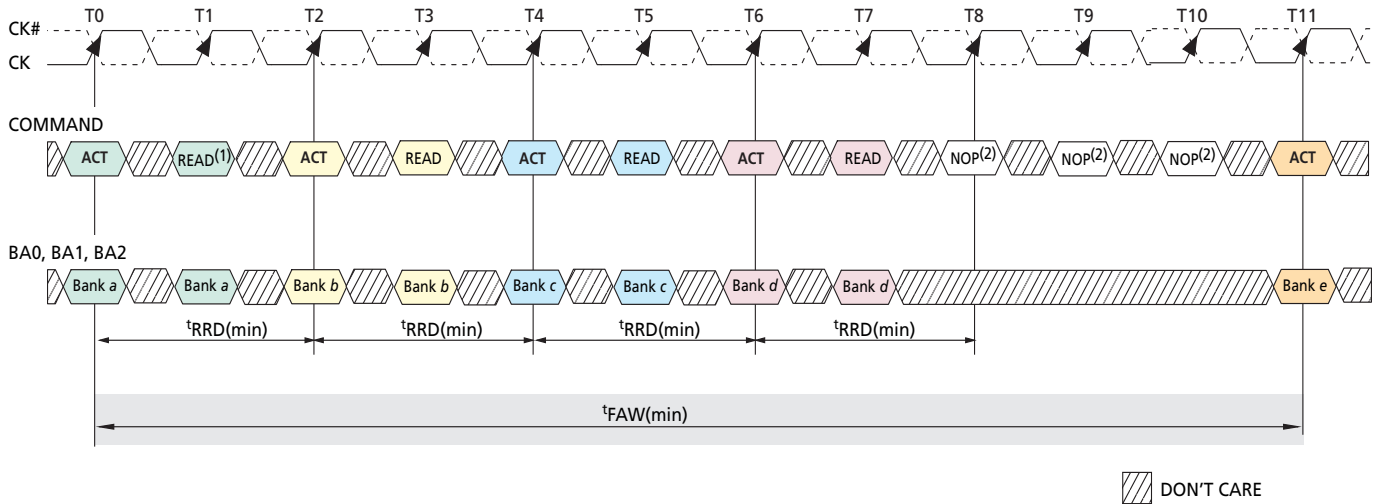
Figure 3: t_{FAW} Example in an 8-Bank Device
