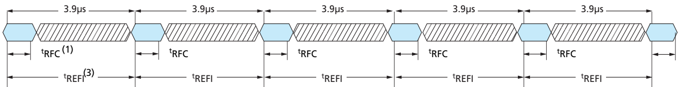
Figure 4: DDR2 Refresh Timing – Optimized for Maximum t_{REFI} Time
