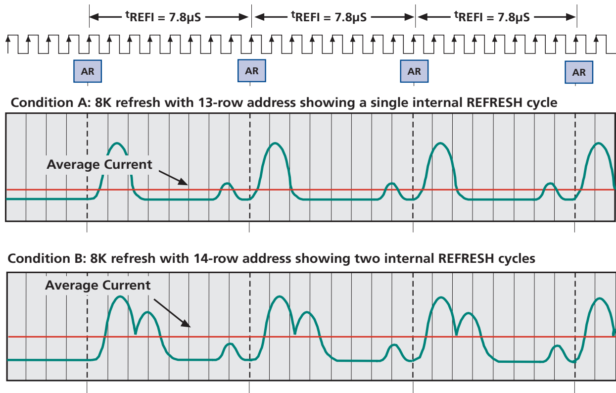
Figure 1: 8K Refresh with 13-Row and 14-Row Addresses
